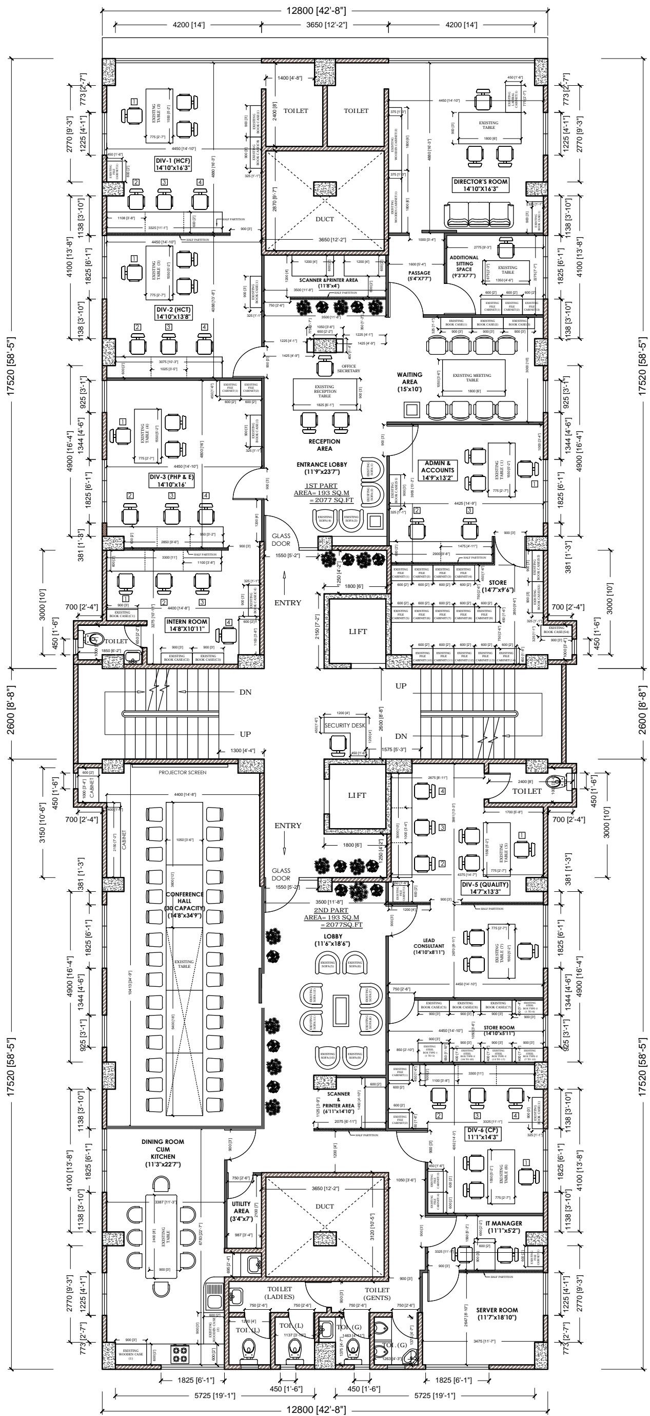
LAYOUT PLAN OF FIRST FLOOR RRC, OFFICE FOR N.E (NHSRC)
